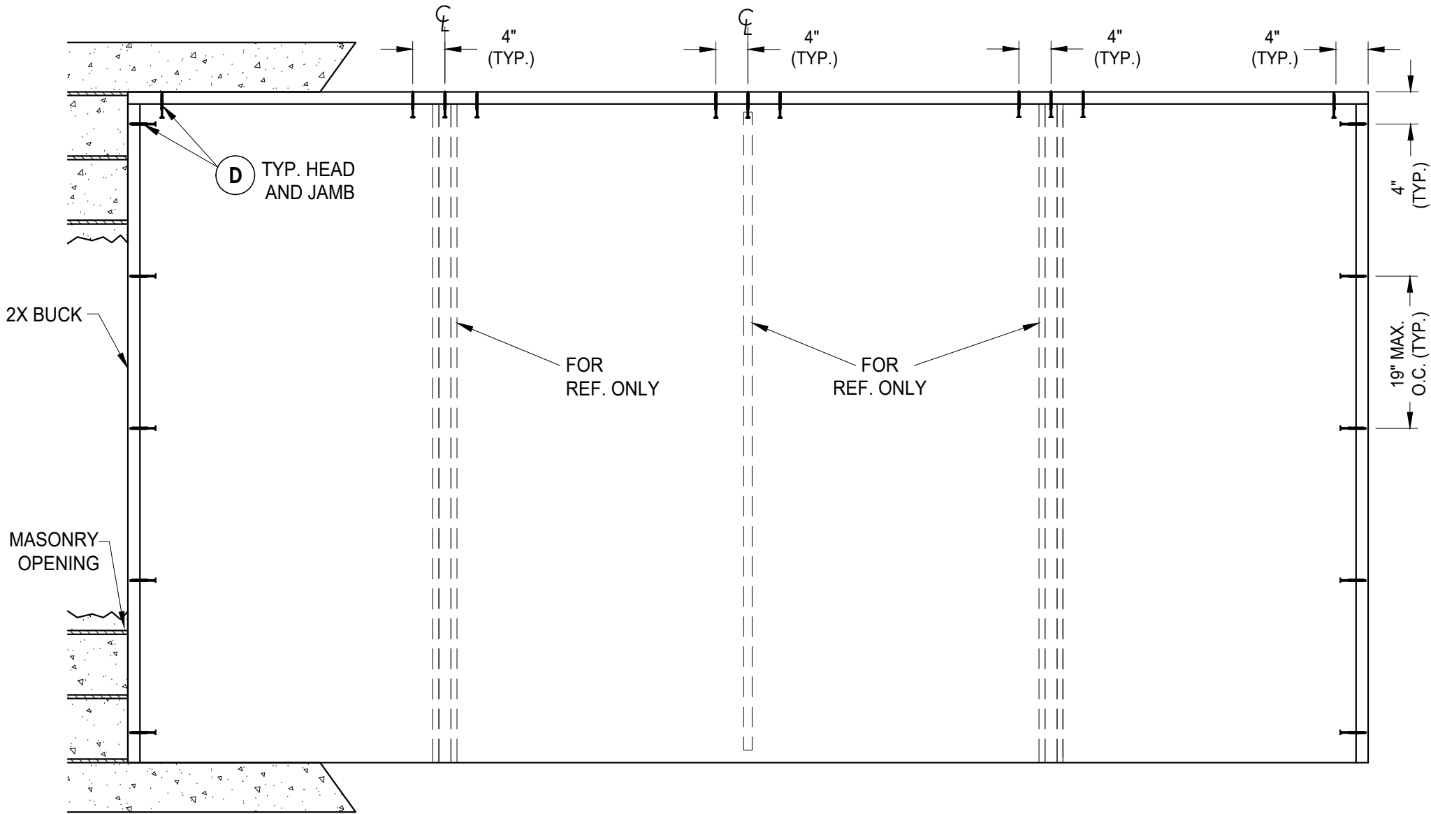
BUCK ANCHORING
