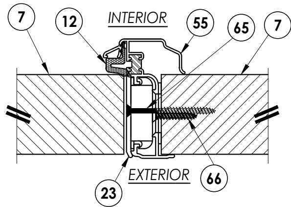
4/4 HORIZONTAL CROSS SECTION Endura astragal
