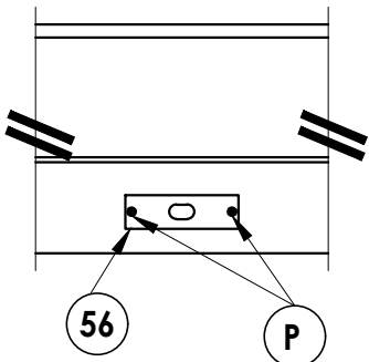
ASTRAGAL STRIKE PLATE "DETAIL 1" - OUTSWING
