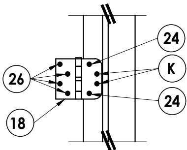
HINGE DETAIL
