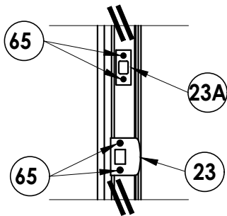
ASTRAGAL DETAIL
