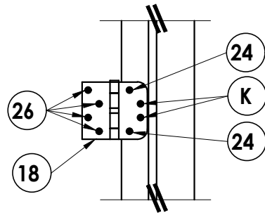
HINGE DETAIL
