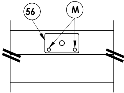
ASTRAGAL STRIKE PLATE "DETAIL 2"
