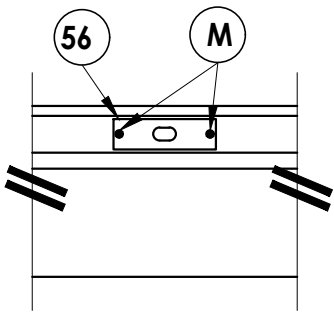
ASTRAGAL STRIKE PLATE "DETAIL 1"- INSWING
